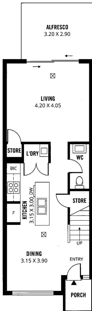
LOWER LEVEL
